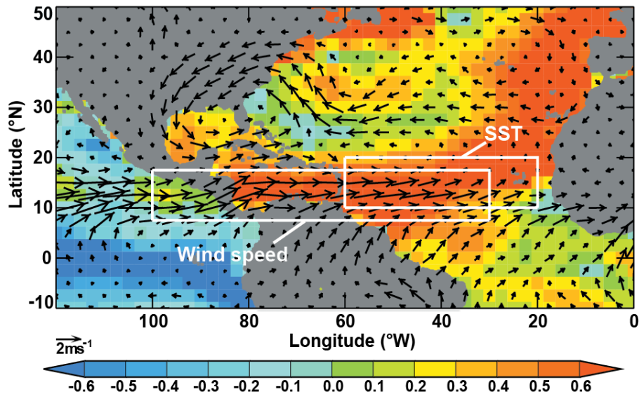
Figure 1. Nature of the TSR statistical model for replicating North Atlantic seasonal hurricane activity. The figure displays the two August-September environmental field areas that the TSR model employs most often in producing a seasonal hurricane outlook. The figure also displays the anomalies in August-September SST (colour coded in °C) and 925 hPa wind (arrowed) linked to active Atlantic hurricane years. Figure taken from Saunders and Lea (2008).
