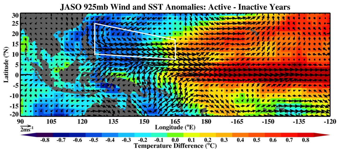
Figure 3. Nature of the physical mechanism behind the TSR primary model in Figure 2. The composite difference figure shows the dominant July-August-September-October (JASO) environmental fields associated with active Northwest Pacific intense typhoon years. Active typhoon seasons occur due to the effects of the anomalous Walker circulation and the resulting weakened easterly trade winds that occur over the tropical Northwest Pacific due to El Niño (warm ENSO) conditions. Inactive typhoon seasons occur due to the effects of the anomalous Walker circulation and the resulting strengthened easterly trade winds that occur over the tropical Northwest Pacific due to La Niña (cold ENSO) conditions. The white quadrilateral denotes where Northwest Pacific tropical cyclones become intense typhoons.
