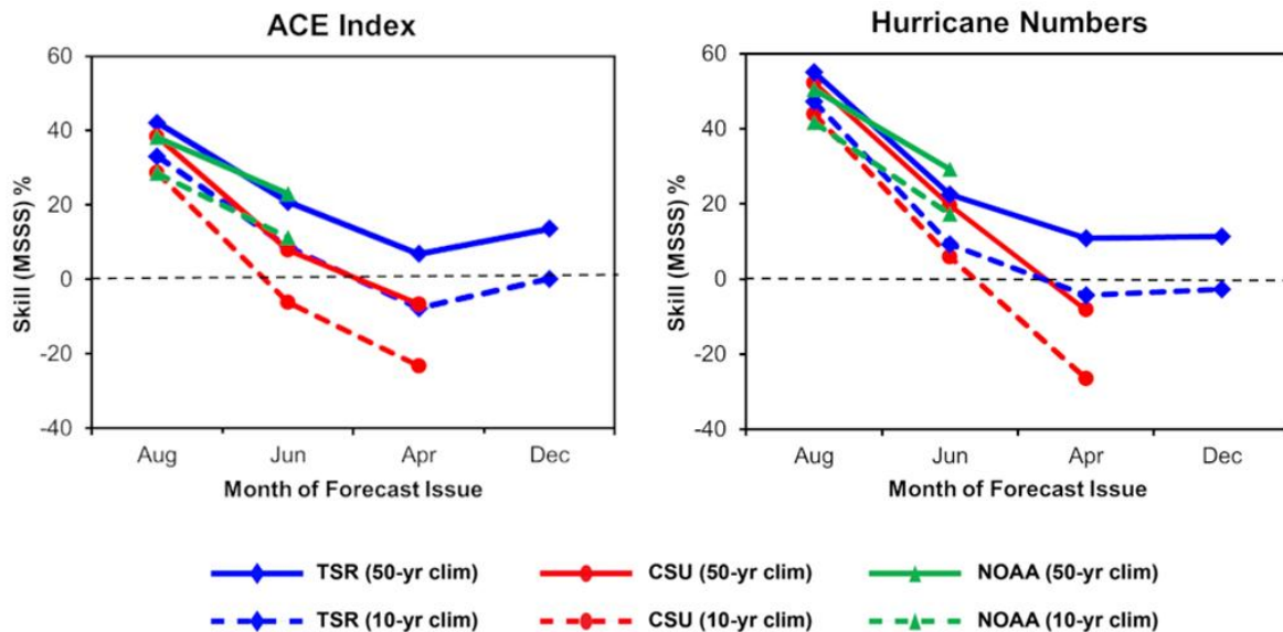
Figure 4. Real-time skill of North Atlantic seasonal tropical cyclone outlooks assessed for the 20-year period 2003-2022. The skill of the seasonal outlooks issued publicly by Tropical Storm Risk (TSR, blue lines), Colorado State University (CSU, red lines), and the National Oceanic and Atmospheric Administration (NOAA, green lines) are compared for ACE (left panel) and for hurricane numbers (right panel). The skill is shown as the Mean Square Skill Score (MSSS) based on a fixed 50-year (1951-2000) climatology and on a running prior 10-year climate norm.
