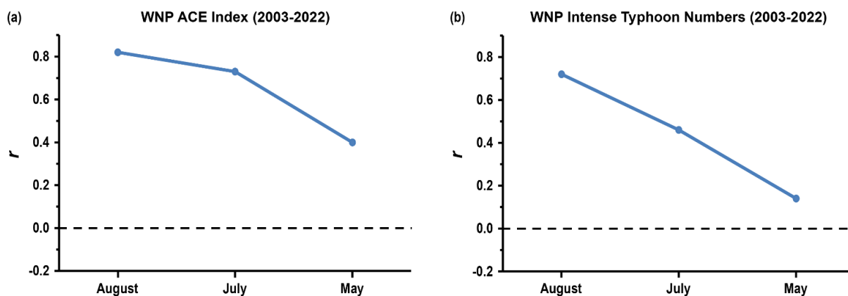
Figure 5. Real-time skill of the TSR seasonal outlooks for northwest Pacific (a) ACE and (b) intense typhoon numbers assessed for the 20-year period 2003-2022. Skill is shown as the Pearson correlation, r , between the forecast values (issued separately in early May, early July and early August) and the observed values.
